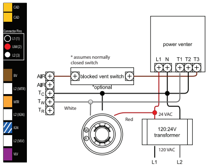
Figure 12 - 24Vac Combustion Air Proving Wiring
