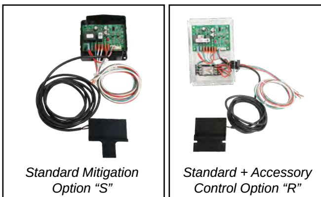
Figure A1 - Mitigation Control Boards (cover removed to show internal components)
